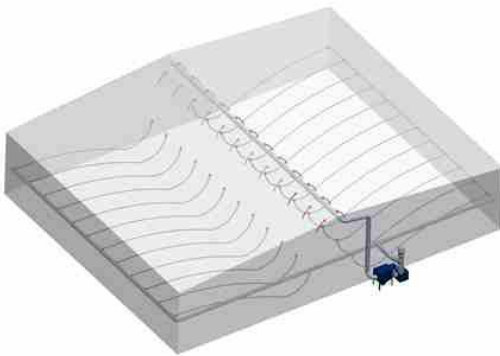
Layer-Blow-Ventilation
